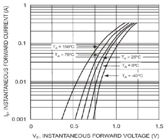
Fig. 1 Forward Characteristics
